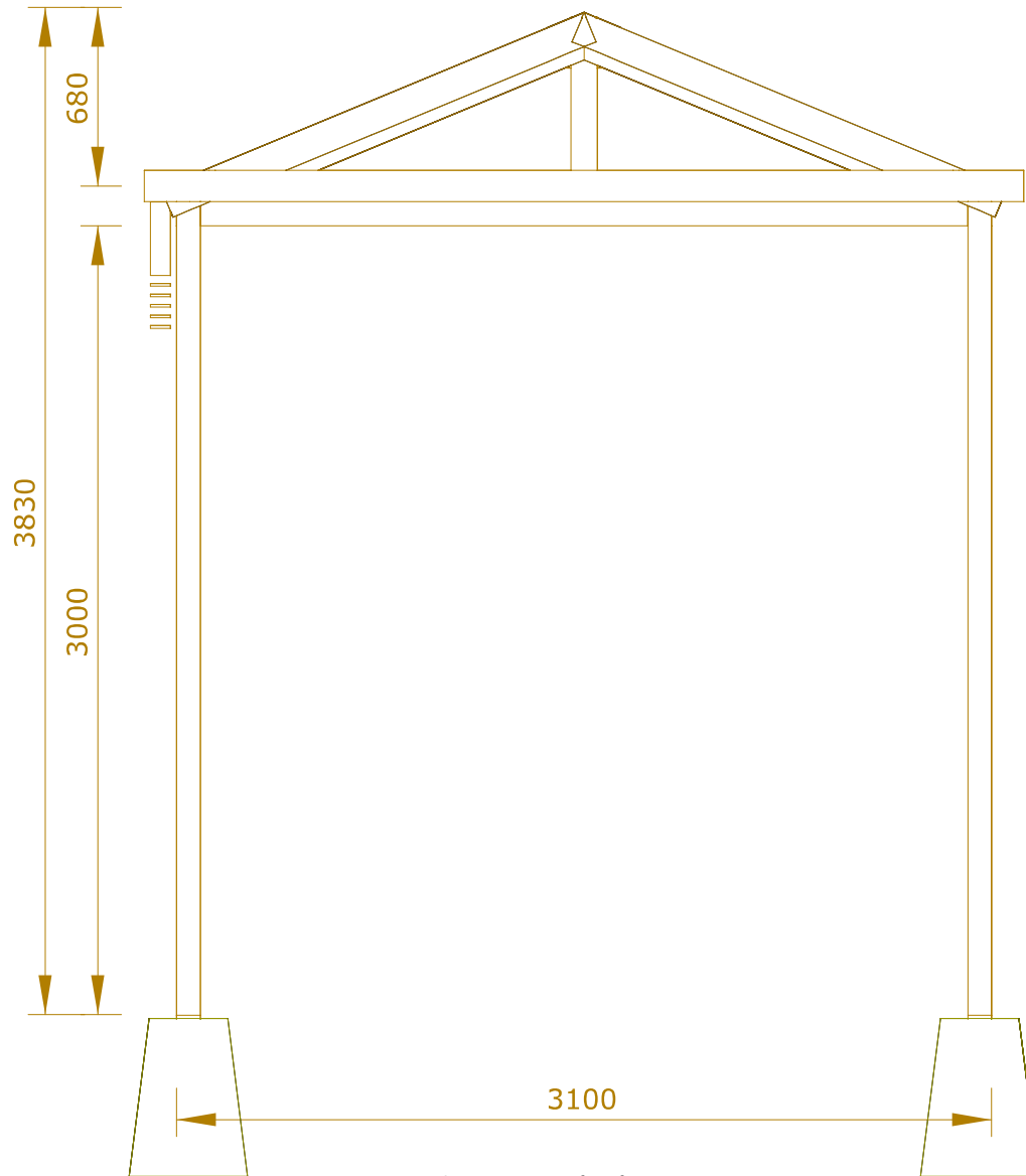
Area 1 - Gable Hip Roof Left Elevation
