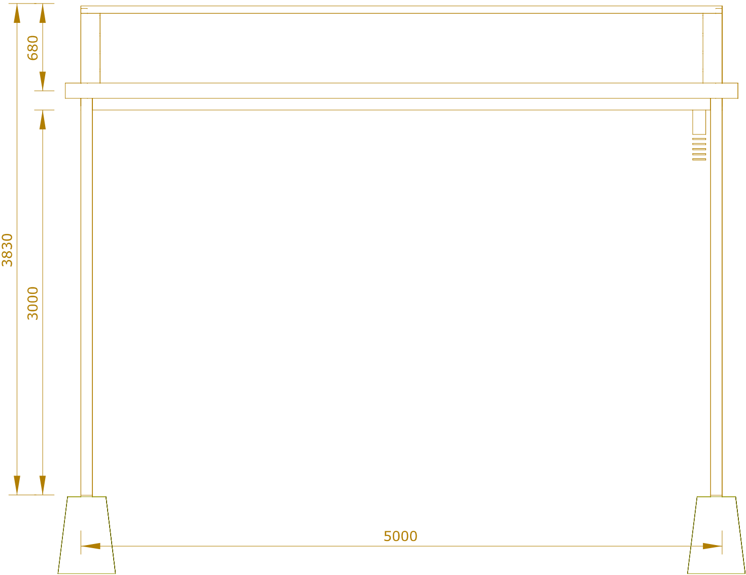
Area 1 - Gable Hip Roof Front Elevation
