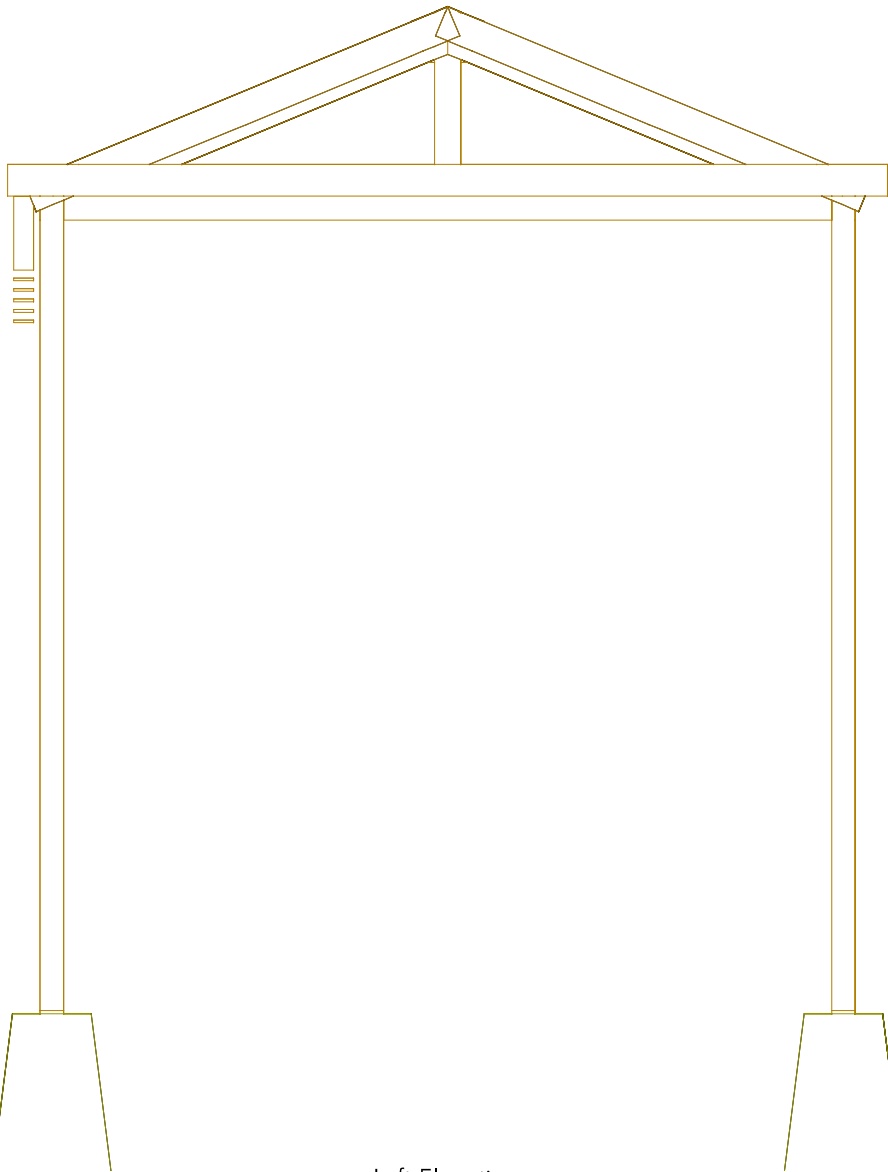
Left Elevation
