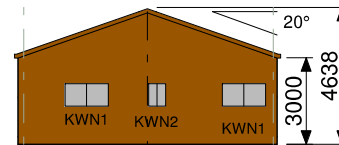
ELEVATION GRID 7
